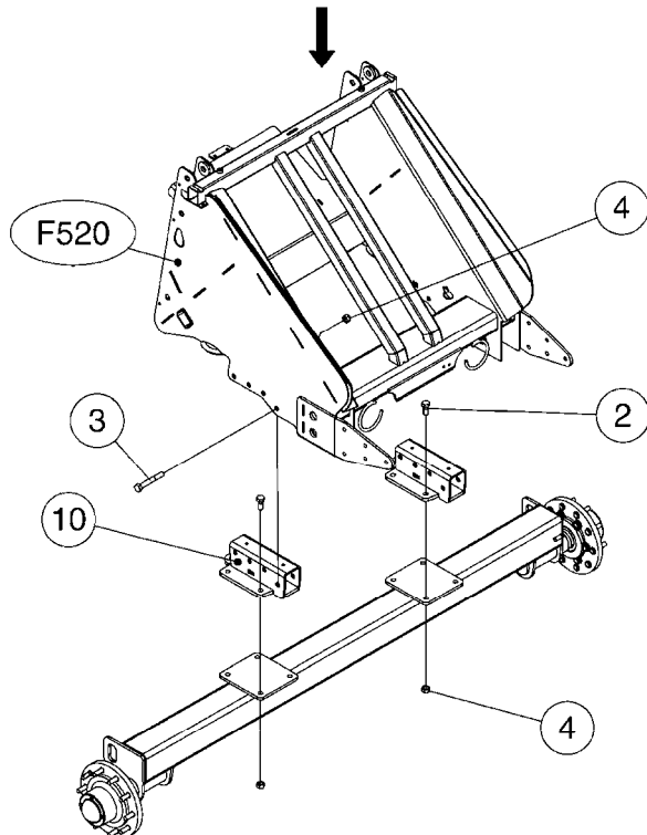
NON SUSPENDED AXLE SYSTEM
